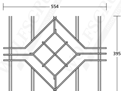
17505-E 12x6
