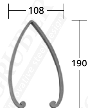
37150 12x6 mm
