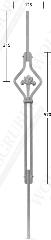
17114 \varnothing 12 mm
