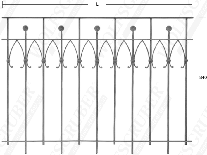
17410 \varnothing 12mm - 20x6 mm - L: 1320 mm
