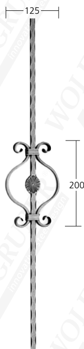
12544 ∅12 mm 1,50 kg
