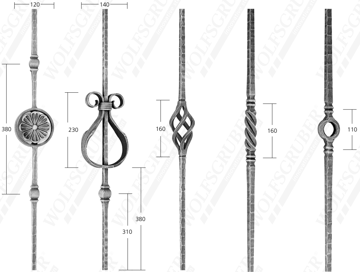
12310 ∅ 14 mm 2,48 kg
