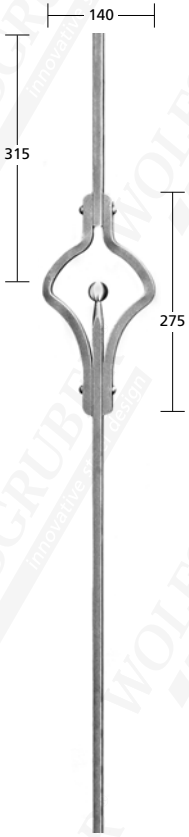
17117 \varnothing 12 mm
