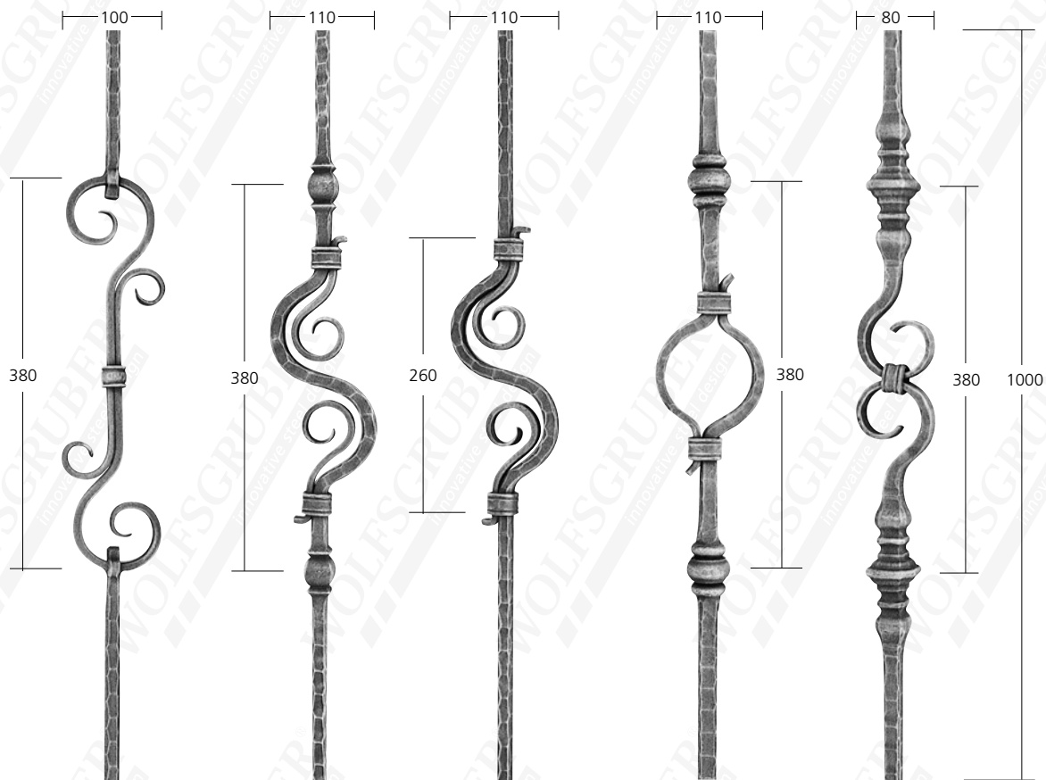
12206 ∅14 mm 1,63 kg
