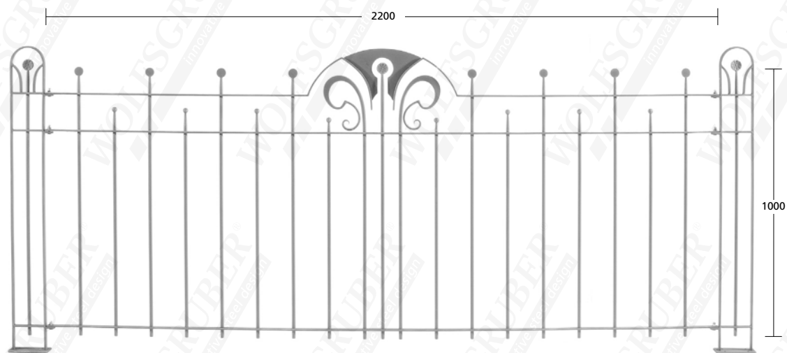
17370 ø 12mm - 20x6 mm
