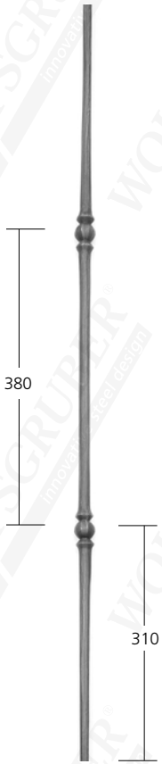
12475 Ø 14-12 mm 1,05 kg
