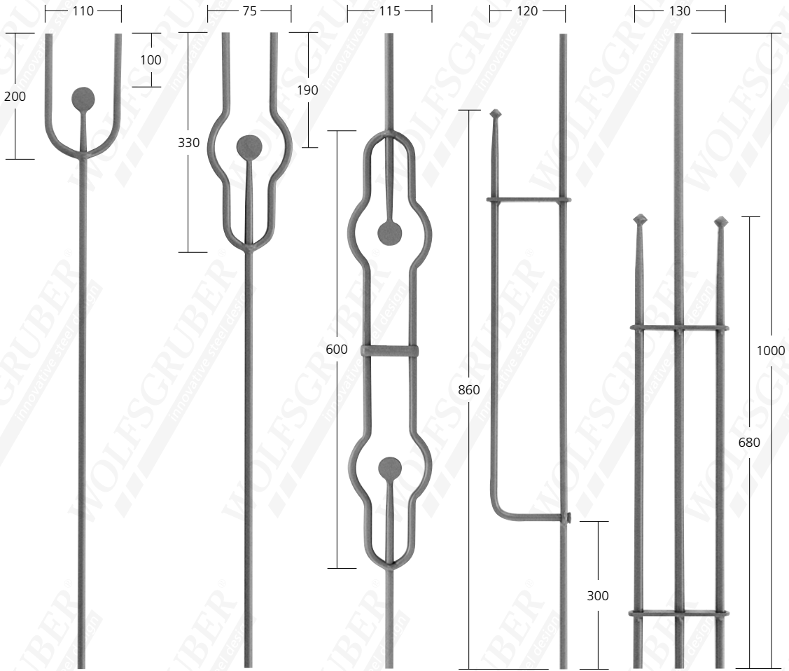
14002 Ø 12 mm 1,18 kg
