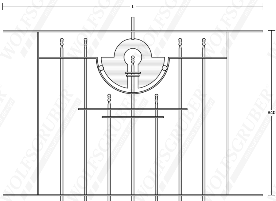
17510 25x8 | \varnothing 12mm - L: 1320
