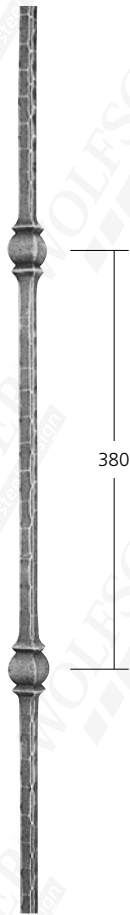
12402 \varnothing 14 mm 1,70 kg
